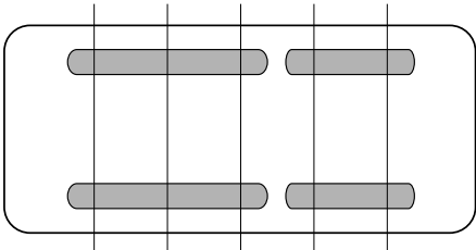
MV52CBJD - 5 string quad coil switchable
